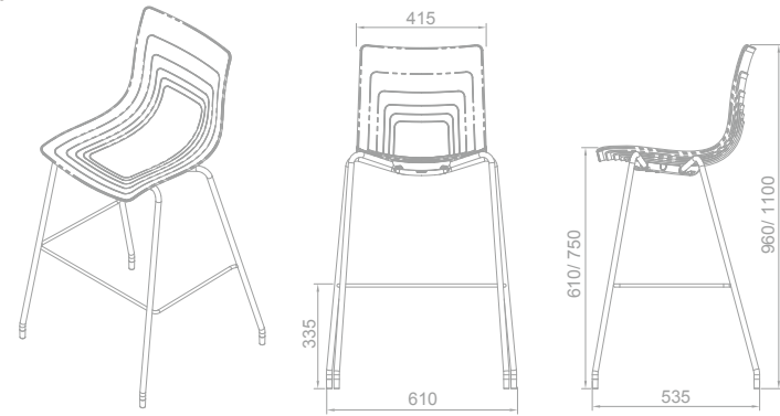
5-WAVES CHAIR Stackable High stool 5W-1H-PP
