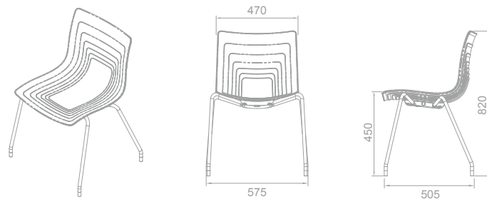
6-WAVES CHAIR Four legs chair 6W-1-PP
