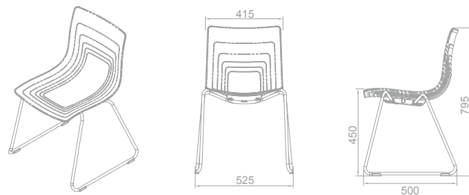
5-WAVES CHAIR Sled base chair 5W-2-PP
